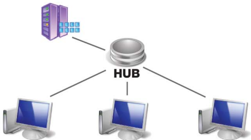
Figure 2: Client/Server Network
